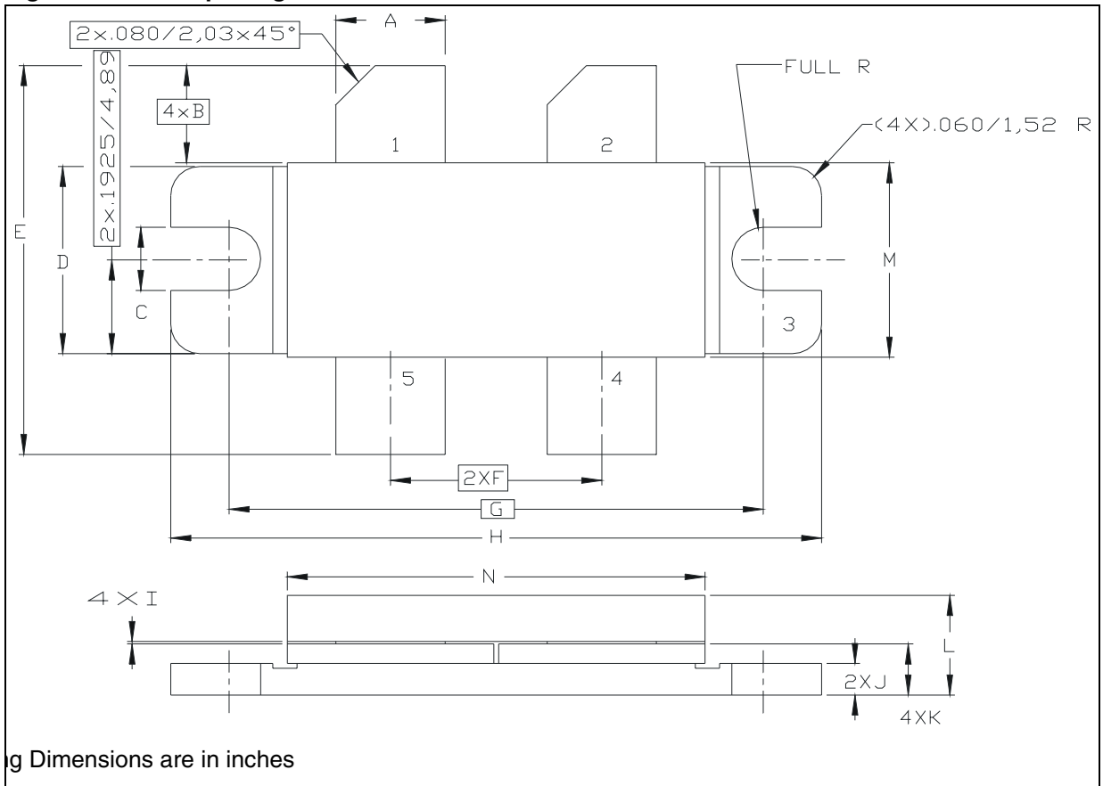
Figure 19. M244 package dimensions
