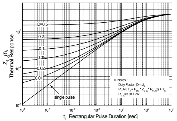
Fig.10 Transient Thermal Response Curve MDF7N65B(TO-220F)
