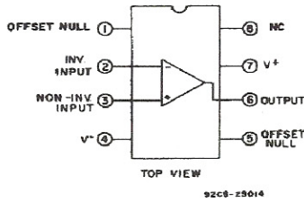
1e.—CA741C and CA741E with internal phase compensation.
