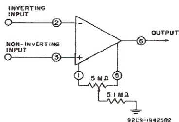
Fig.10—Voltage-offset null circuit for CA748C and CA748.
