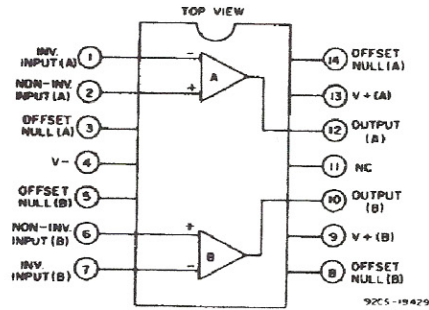
1f.—CA747CE and CA747E with internal phase compensation.
