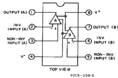
1h.—CA1458E and CA1558E with internal phase compensation.
