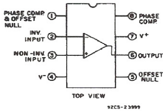
1g.—CA748CE and CA748E with external phase compensation.
